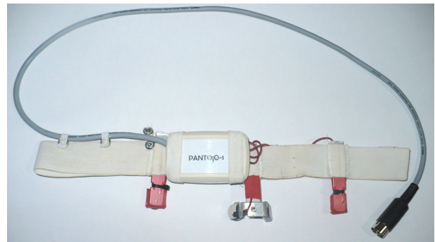
Fig. 2. Head-band of PANTOJO. Note the amplifier circuit is located only a few centimetres away from the electrodes. The central electrode is applied on the nasal septum and the two lateral electrodes on the temples, one for EOG of the healthy eye, the other as electrical reference.
